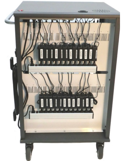
Rear door: inside view of QUICK→SET cable management
